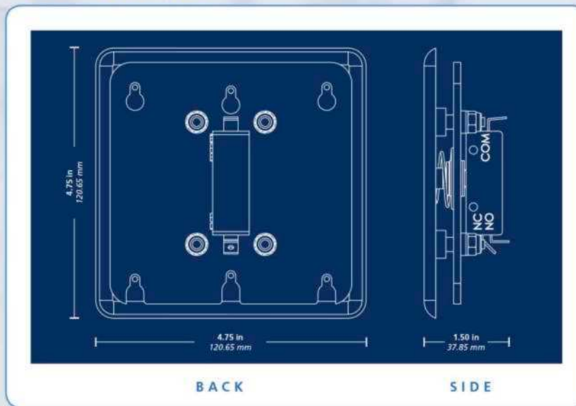
10WRSQ475 4 3/4 inch Weather Ring
